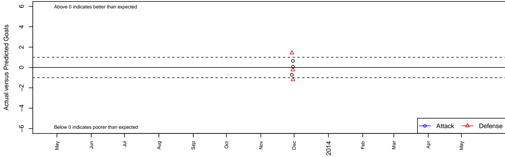
FC Golden State Black G00 Dots are actual minus expected GF (blue circles) and GA (red triangles). Blue line is smoothed change in attack strength. Red is smoothed change in defense strength.
